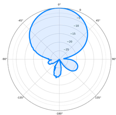
A2010 XZ Plane
